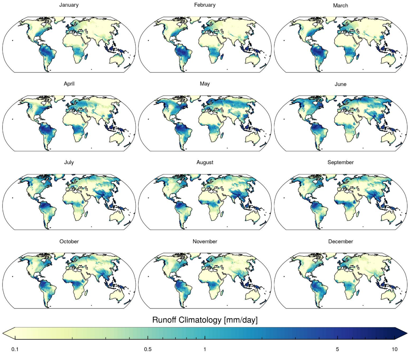
Supplementary Figure 1: Runoff monthly climatology for the period 1971-2010.
